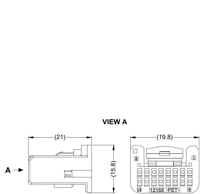
16 PIN FEMALE MATING FACE CONNECTOR - 1318386-1 PIN - 1123343-1
